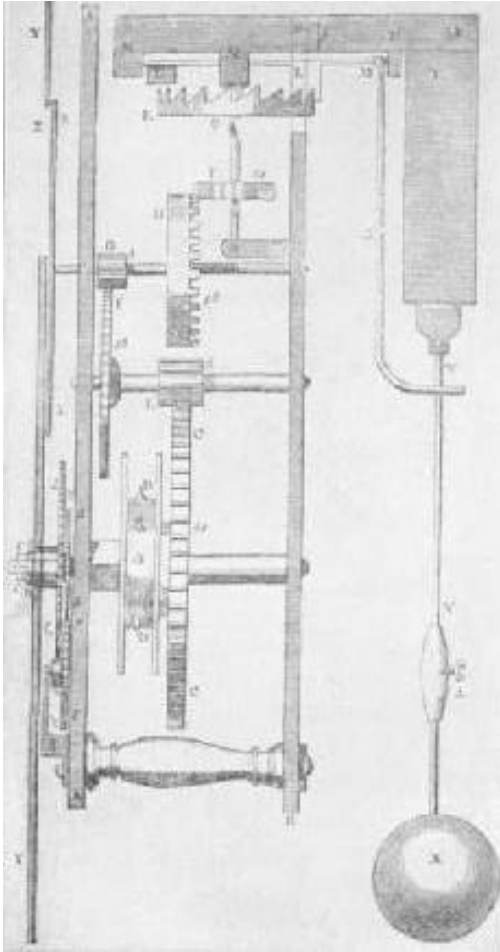
HUYGENS'S CLOCK
